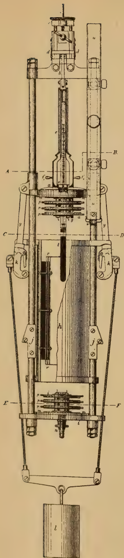
FIG. 6.—NANSEN-PETERSSON WATER-BOTTLE (OPEN).
